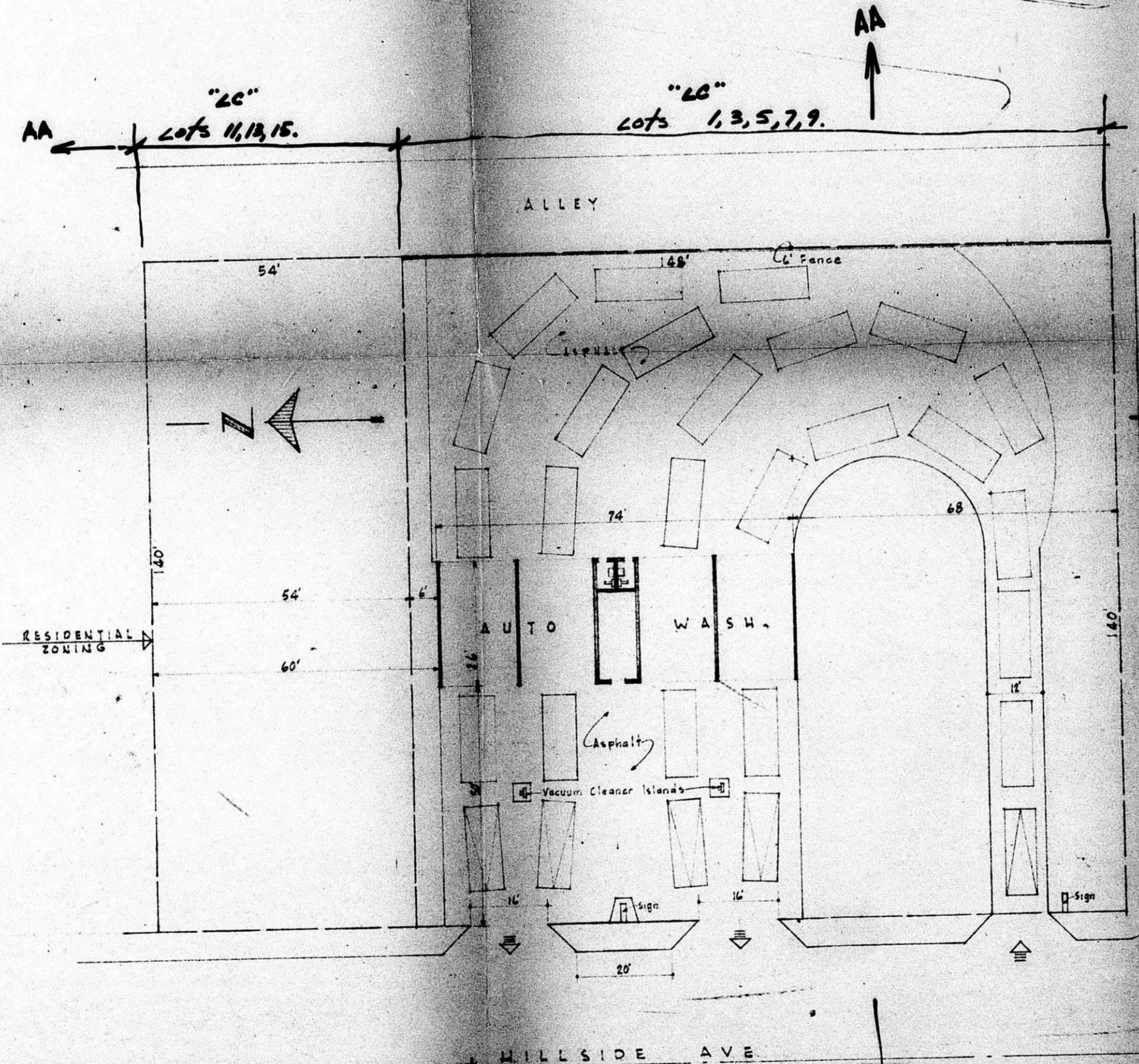
PLOT PLAN 1" = 16'-0"
