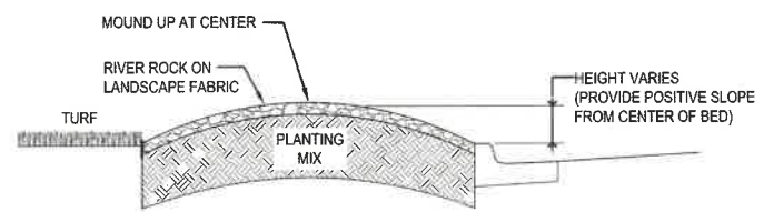
TYPICAL PLANTING BED DIAGRAM NOT TO SCALE
