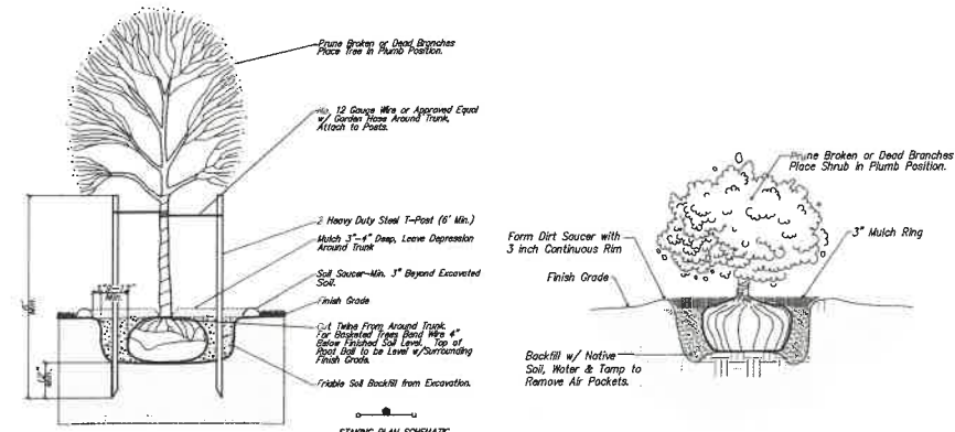
1 TREE PLANTING & STAKING DETAIL No Scale 2 SHRUB PLANTING DETAIL No Scale
