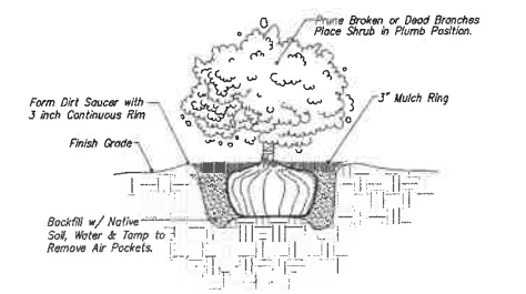
2 SHRUB PLANTING DETAIL No Scale
