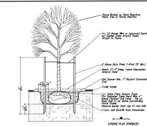
1 TREE PLANTING & STAKING DETAIL No Scale
