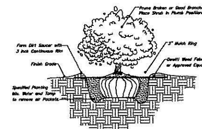
SHRUB PLANTING DETAIL 3 Galon and Smaller No Scale
