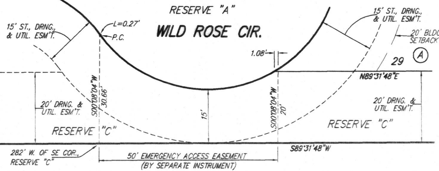
DETAIL "B" (NO SCALE)
