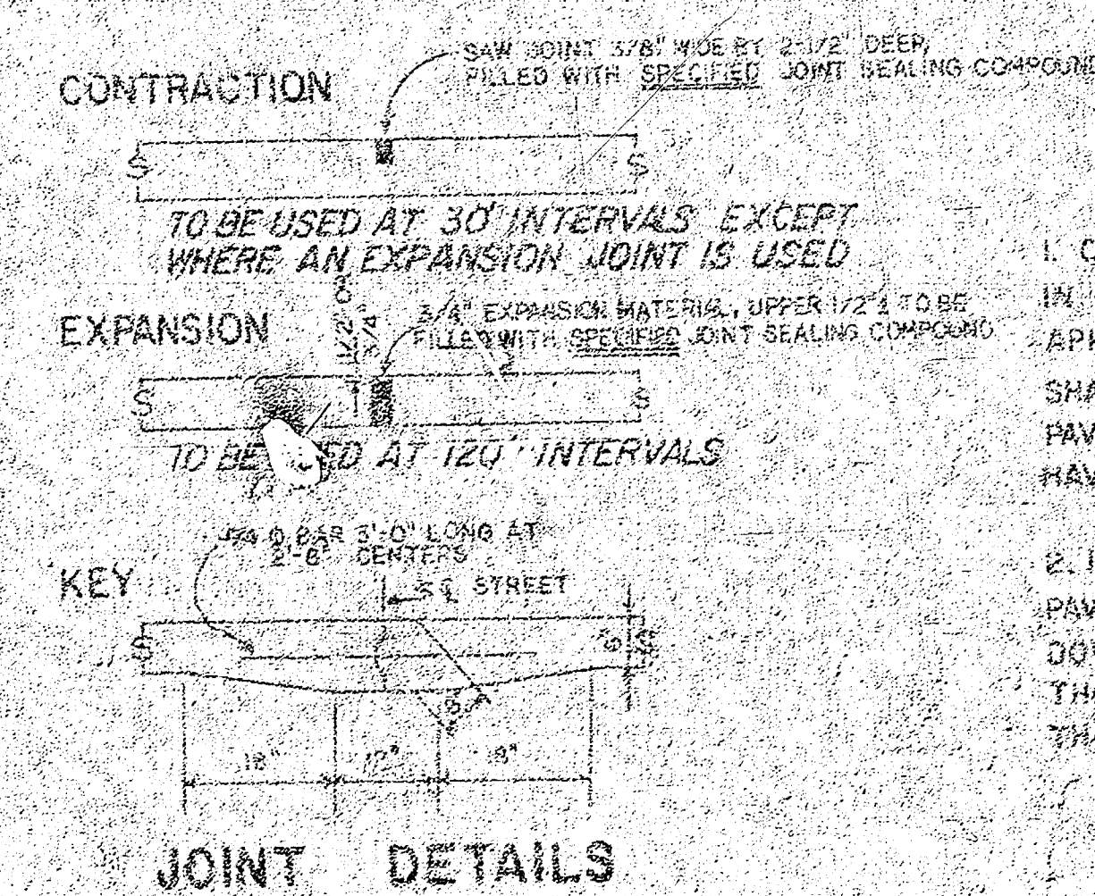
JOINT DETAILS
