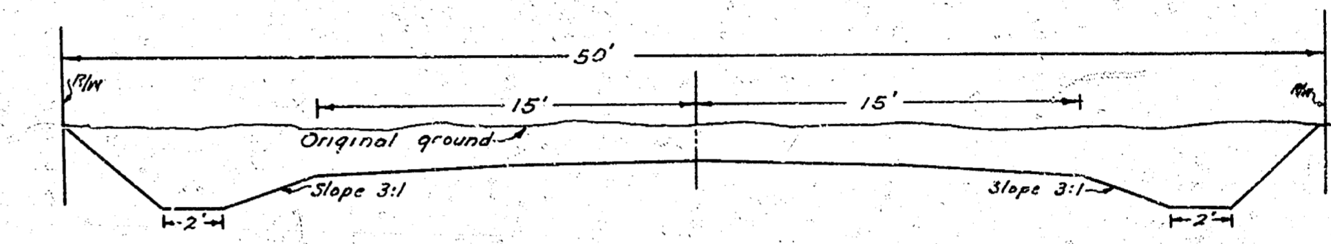
TYPICAL SECTION THRU CUT Scale 1"=5'
