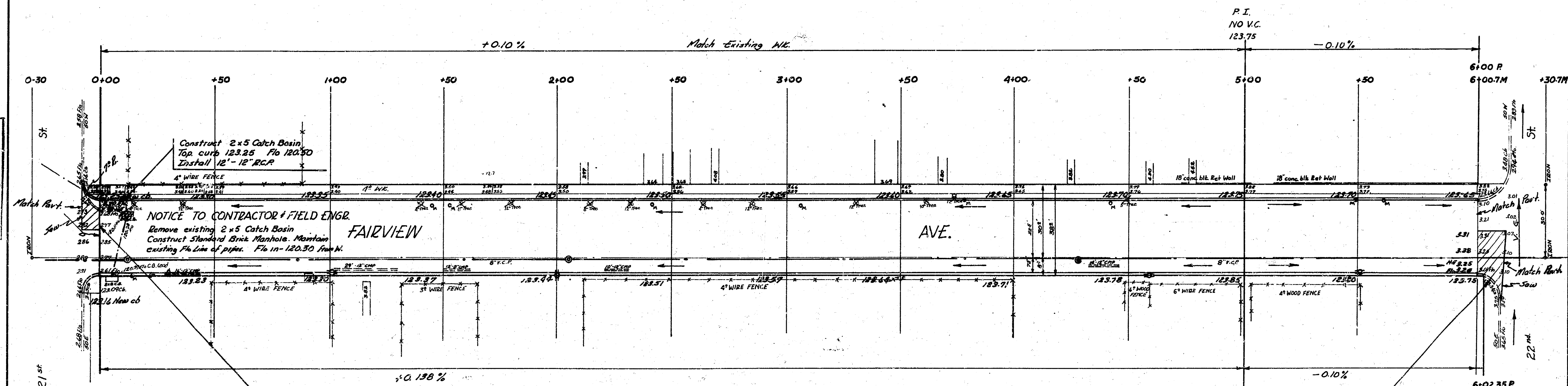
DETAIL OF RAMP W.S. FAIRVIEW
