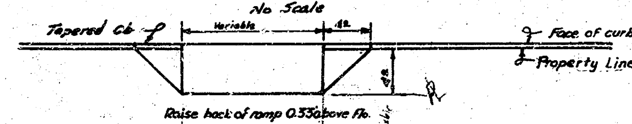
DETAIL OF RAMP E.S. FAIRVIEW
