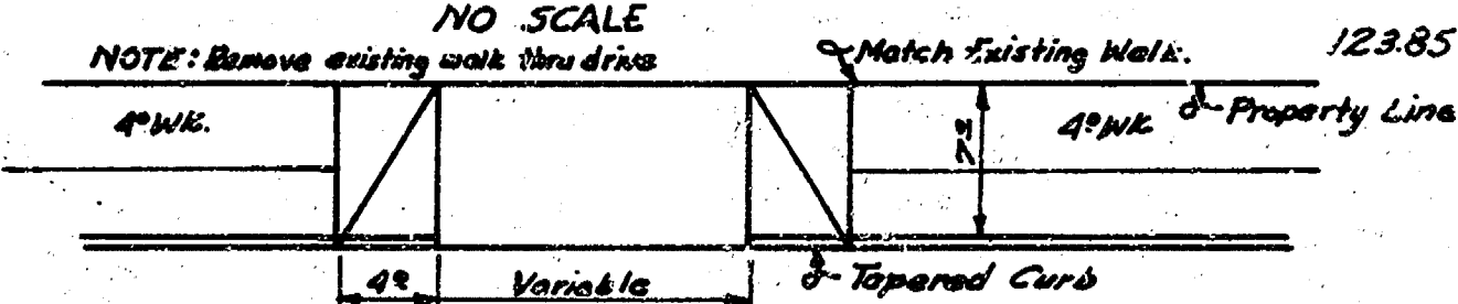
DETAIL OF RAMP W.S. FAIRVIEW
