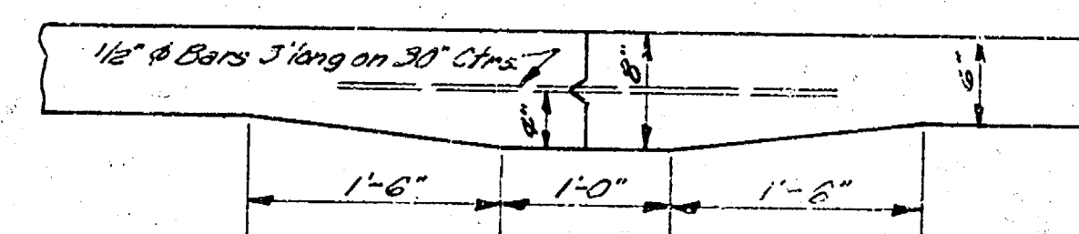
Mastic Joint Detail No Scale
