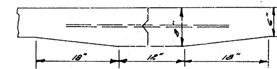
Use 1/2" # 2 Bars, 3' Long, on 2'-6" Ctrs. Mastic Joint Detail
