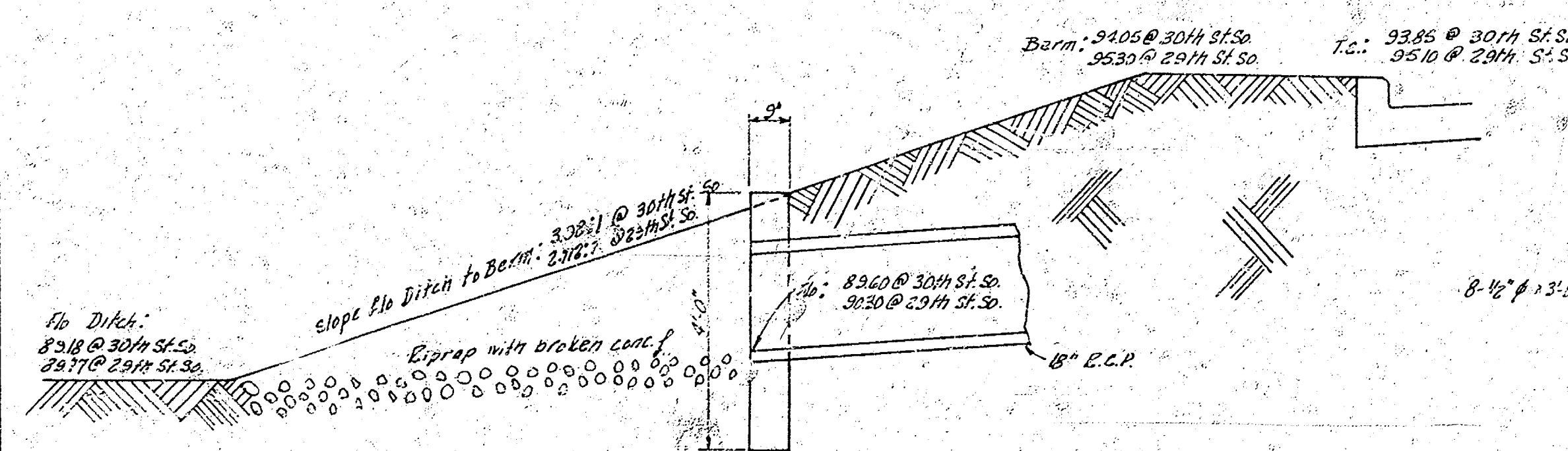
SECTION THRU BANK AT HEADWALL NOT TO SCALE
