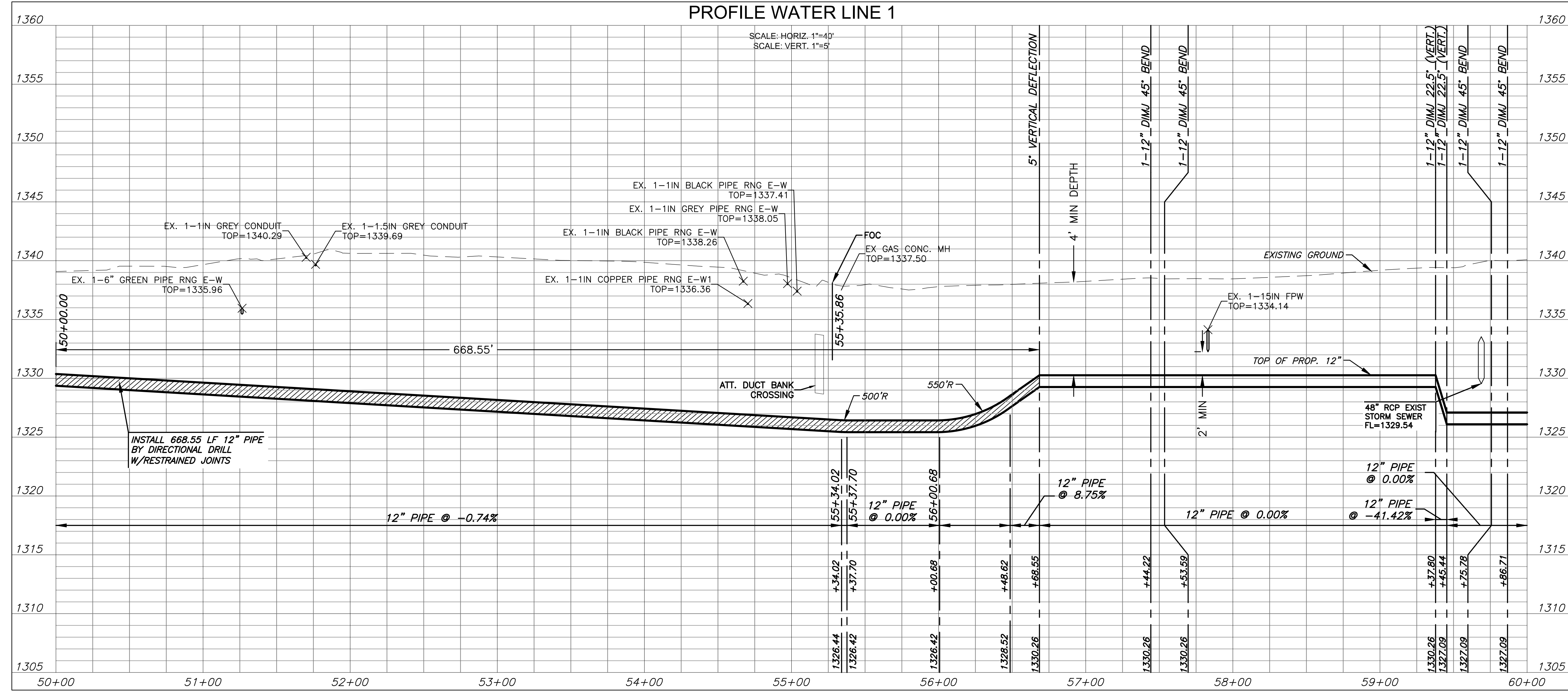
PLAN WATER LINE 1 PROFILE WATER LINE 1
