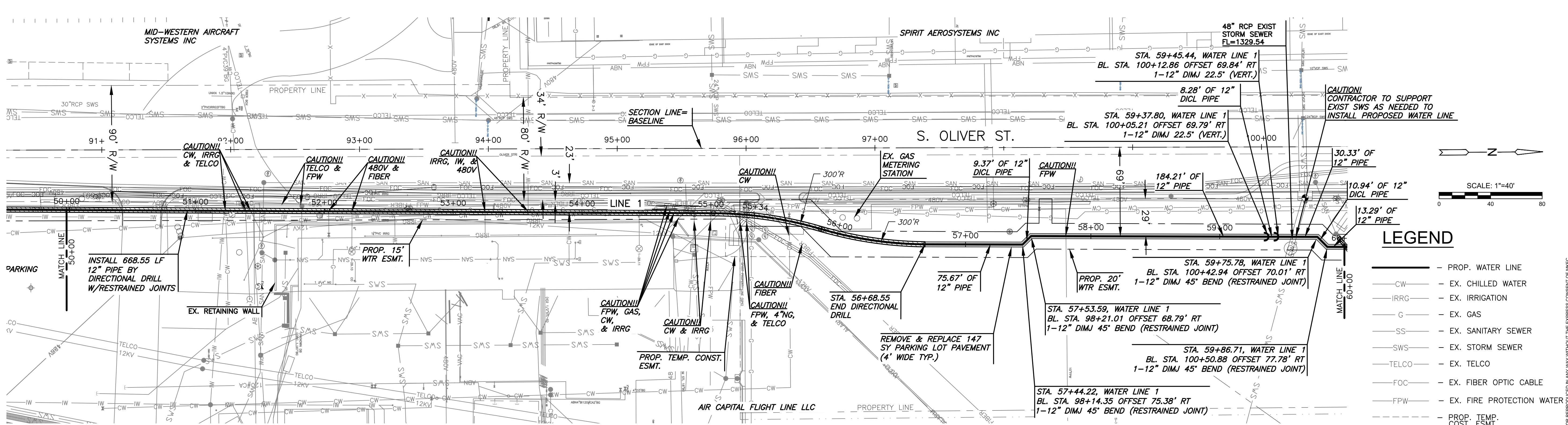
PLAN WATER LINE 1 PROFILE WATER LINE 1
