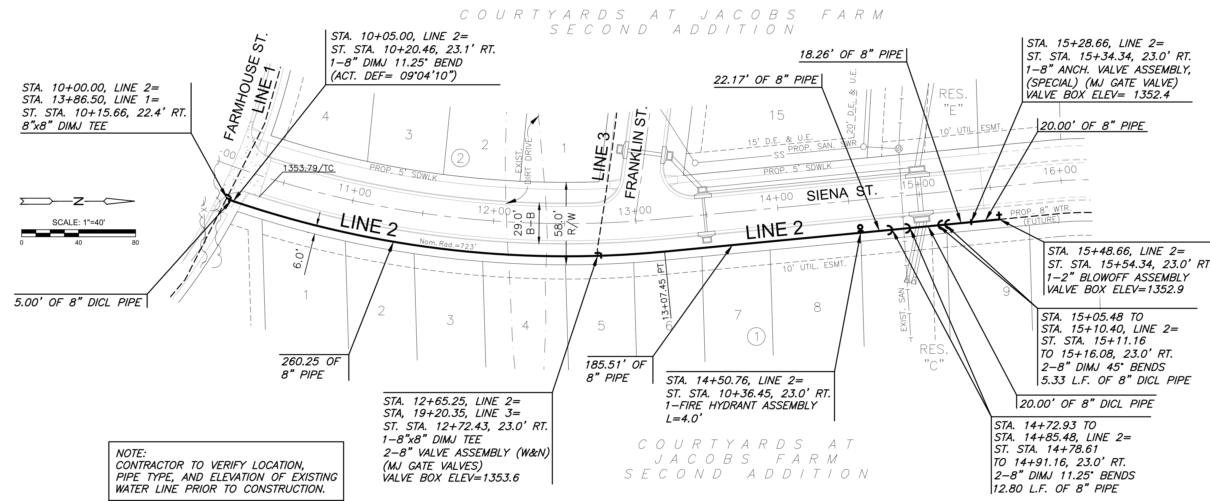
PLAN WATER LINE 2
