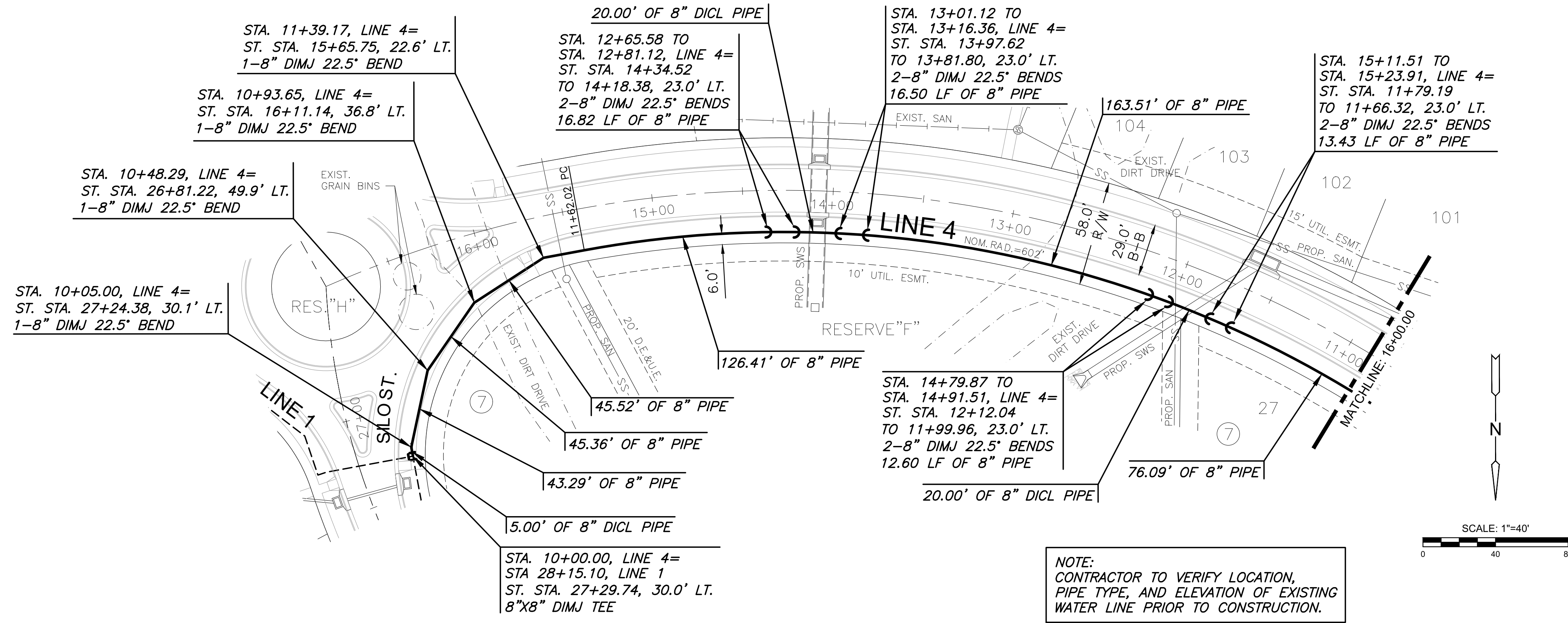
PLAN WATER LINE 4 (10+00.00 - 16+00.00)
