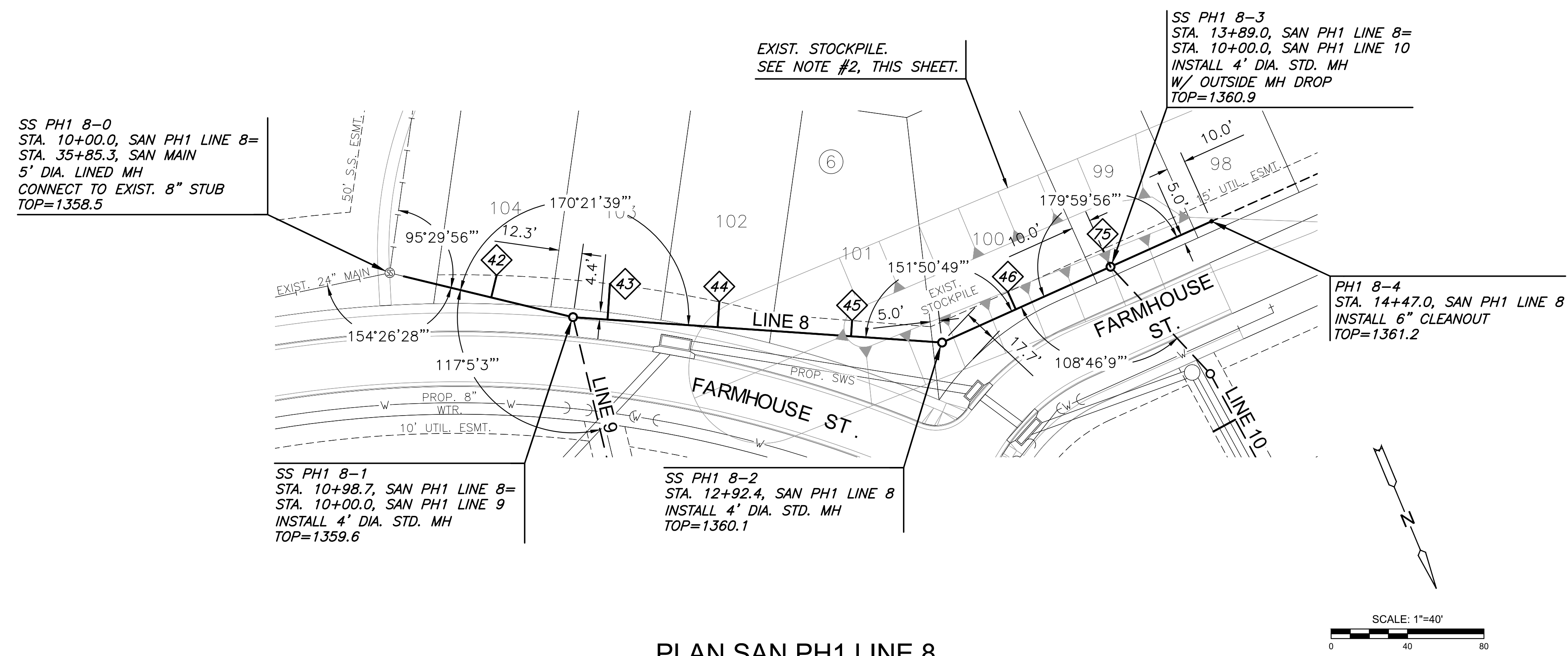
PLAN SAN PH1 LINE 8 PROFILE SAN PH1 LINE 8
