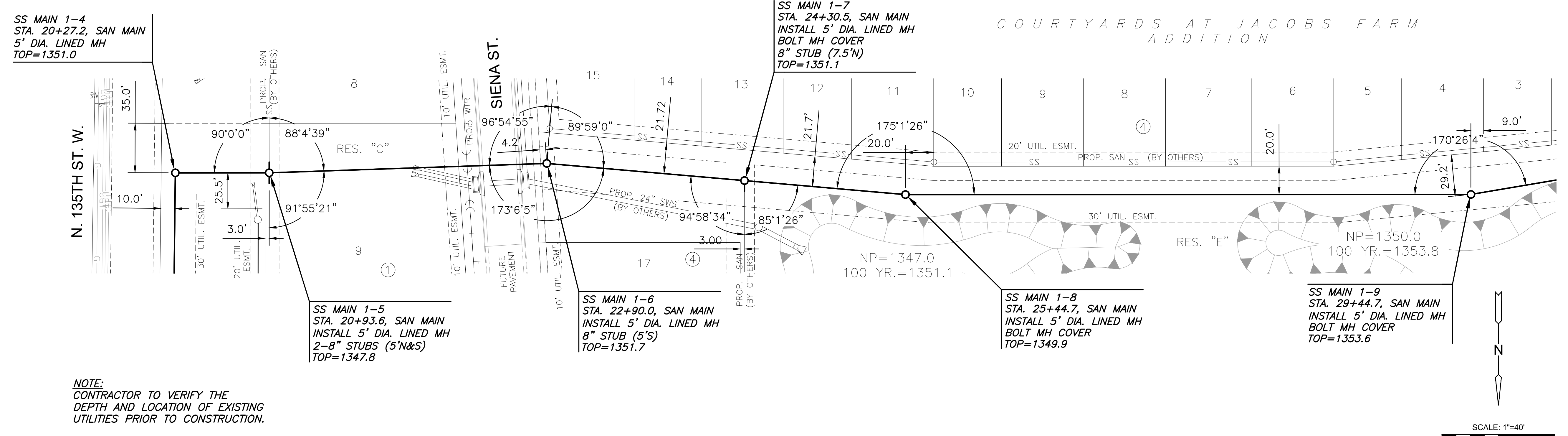
PLAN SAN MAIN LINE (20+27.2 - 29+44.7) PROFILE SAN MAIN LINE (20+27.2 - 29+44.7)
