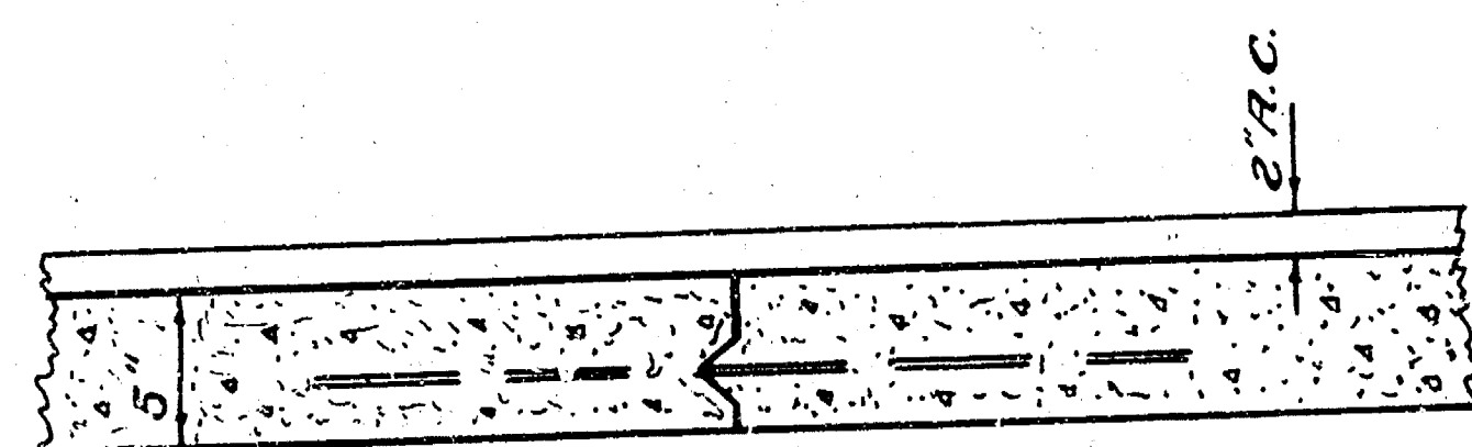
DETAIL of KEYED JOINT no scale
