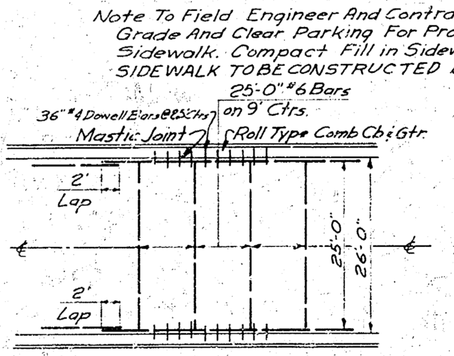
TYPICAL STEEL PATTERN
