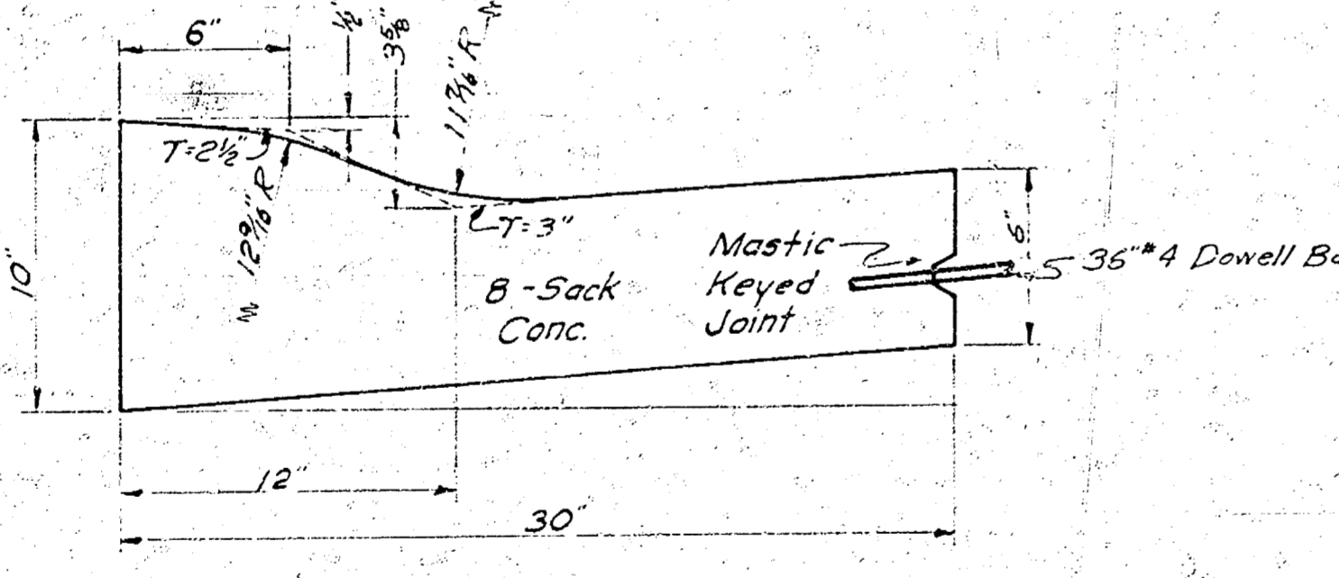
ROLL CURB DETAIL
