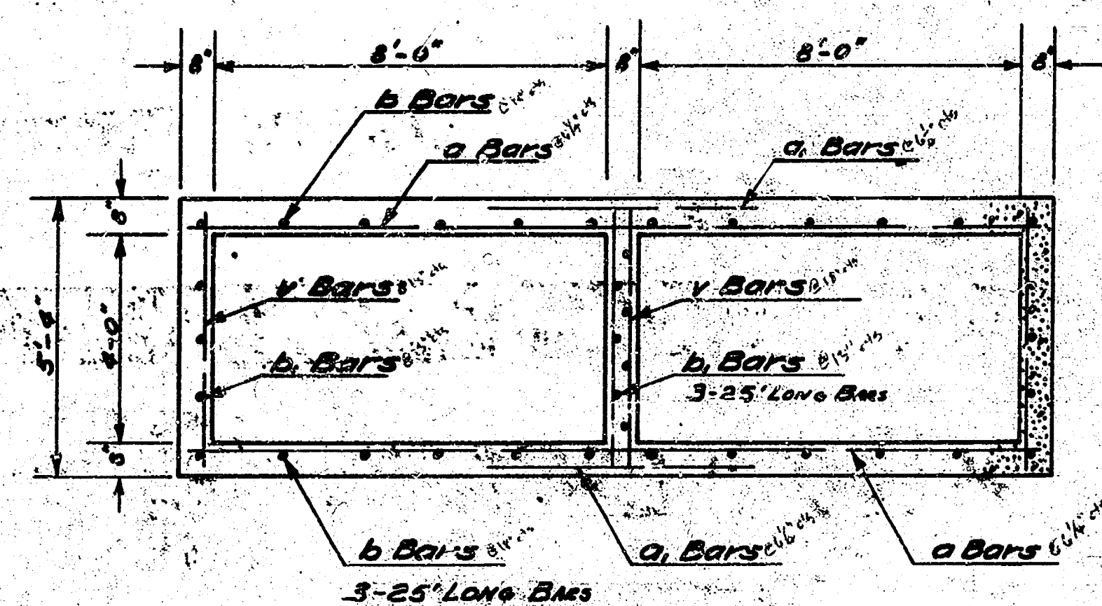
CROSS SECTION OF DOUBLE 8' BOX
