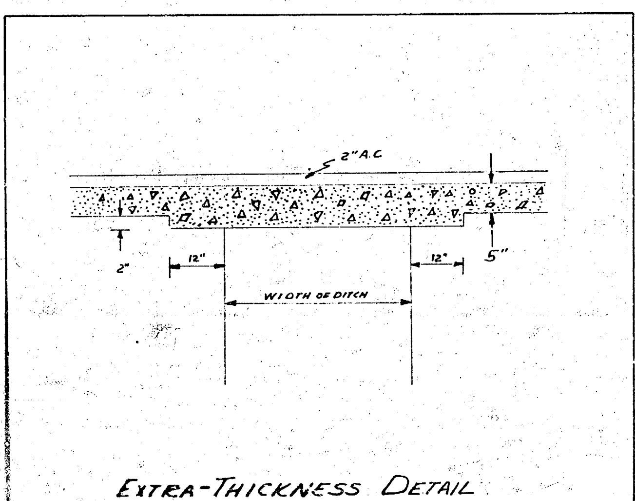
EXTRA-THICKNESS DETAIL
