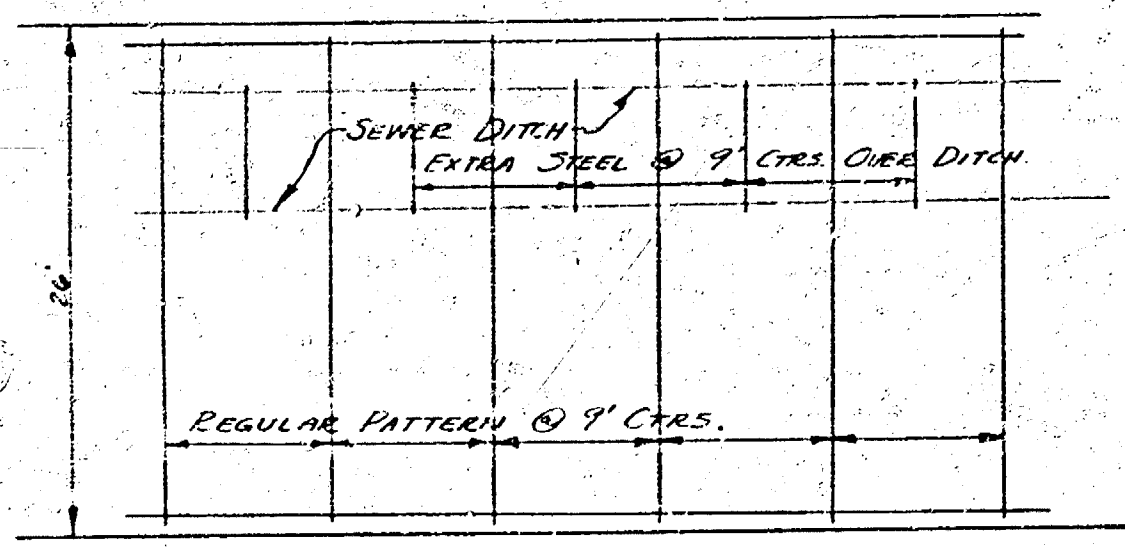
STEEL DETAIL
