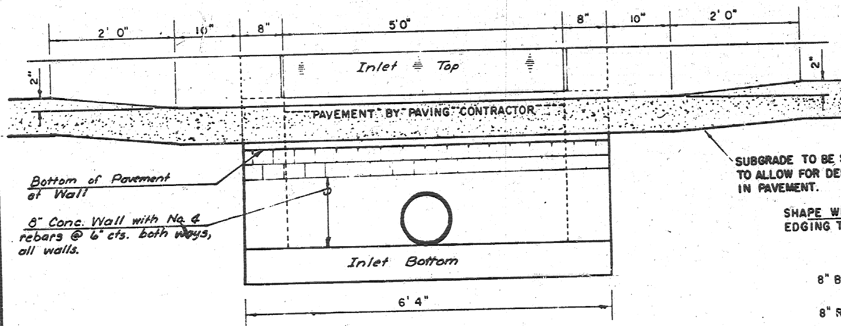
SECTION C-C
