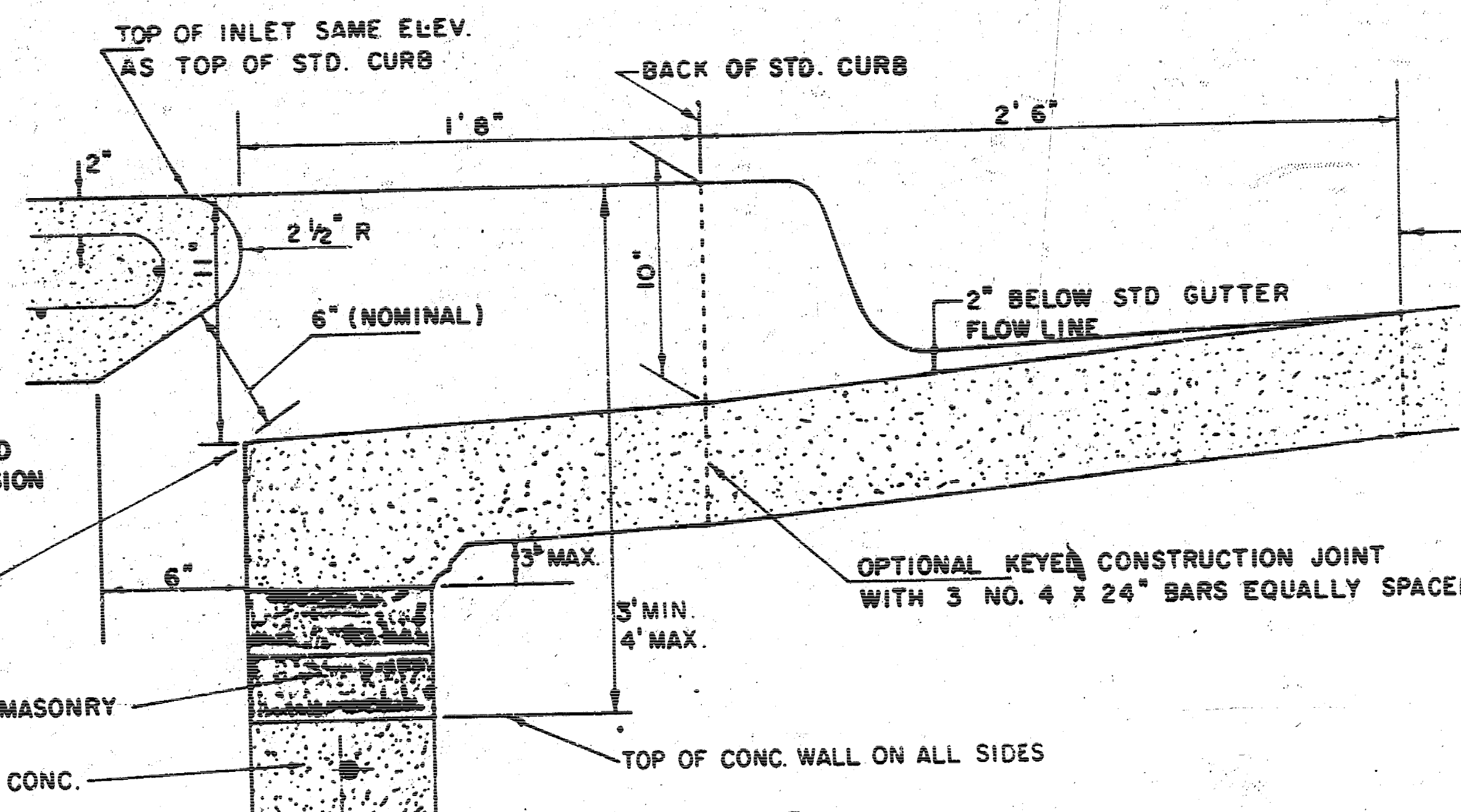
SECTION B-B
