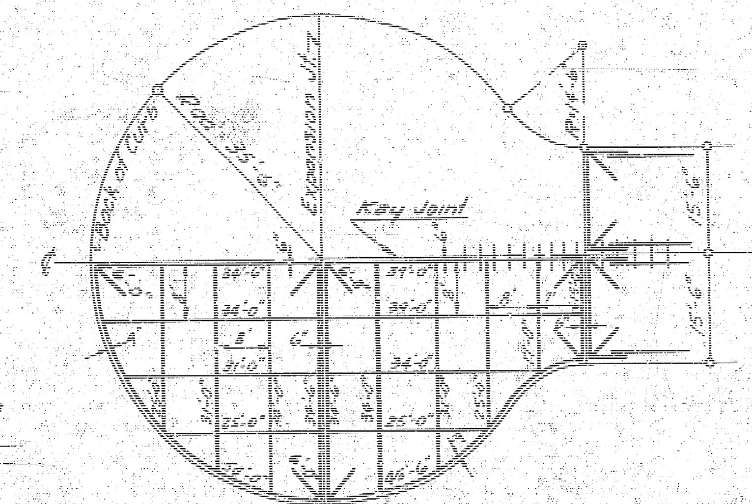
CONCRETE CUL-DE-SAC STEEL PATTERN No Scale
