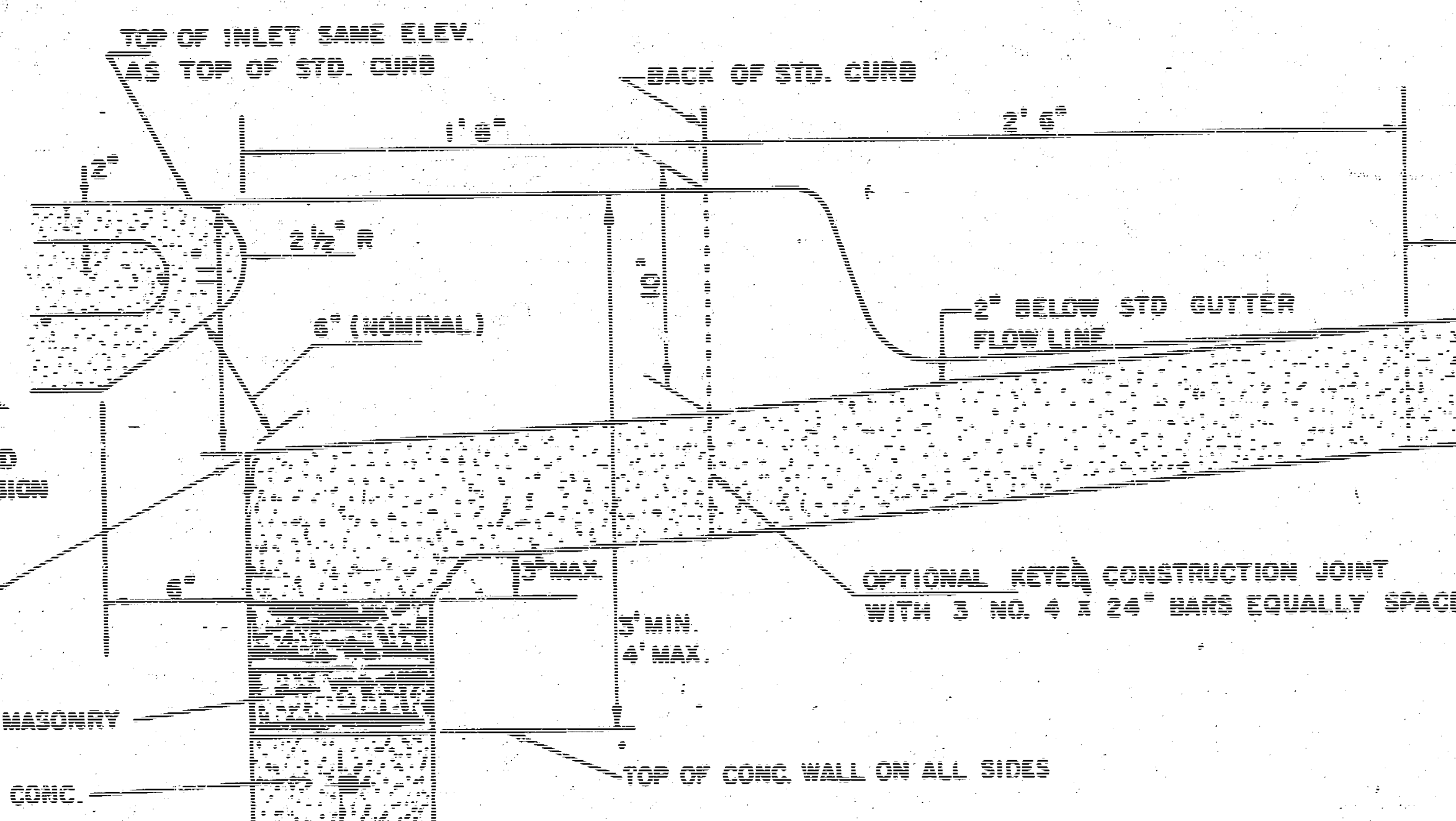
SECTION B-B
