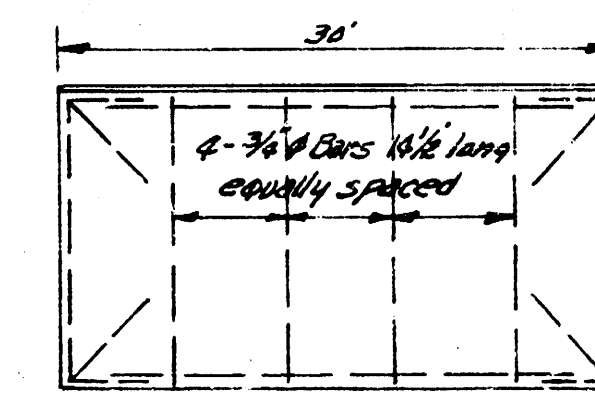
Steel Pattern for W.B. Foot between Alturas and Hamilton. No Scale
