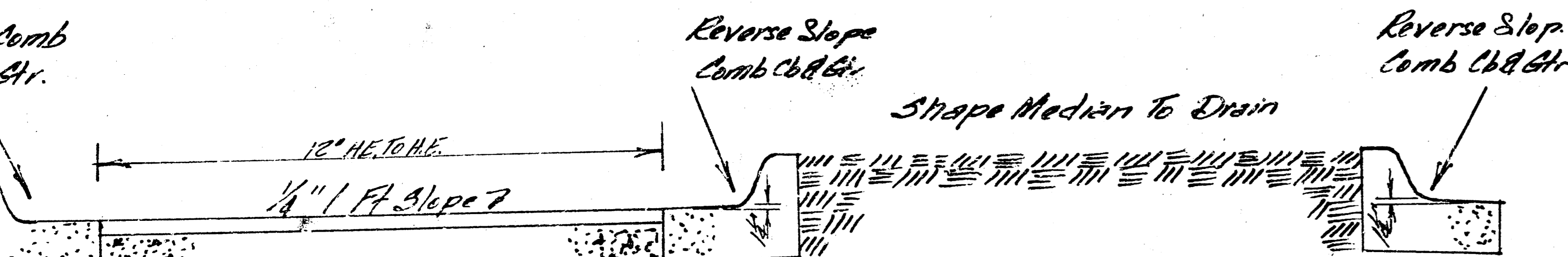
TYPICAL HALF SECTION No Scale
