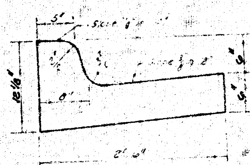
ROAD SIDE CURB & GUTTER
