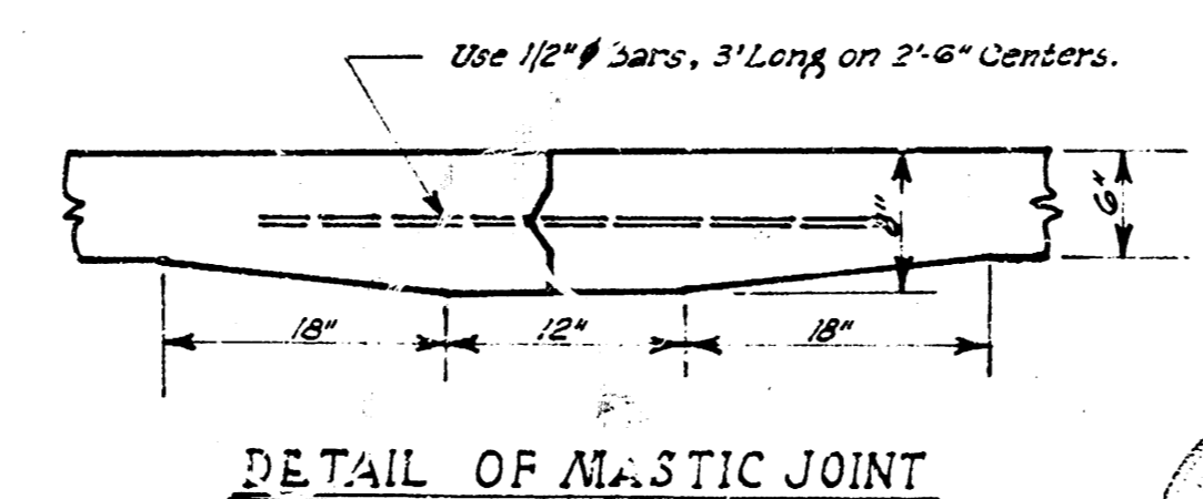
DETAIL OF MASTIC JOINT
