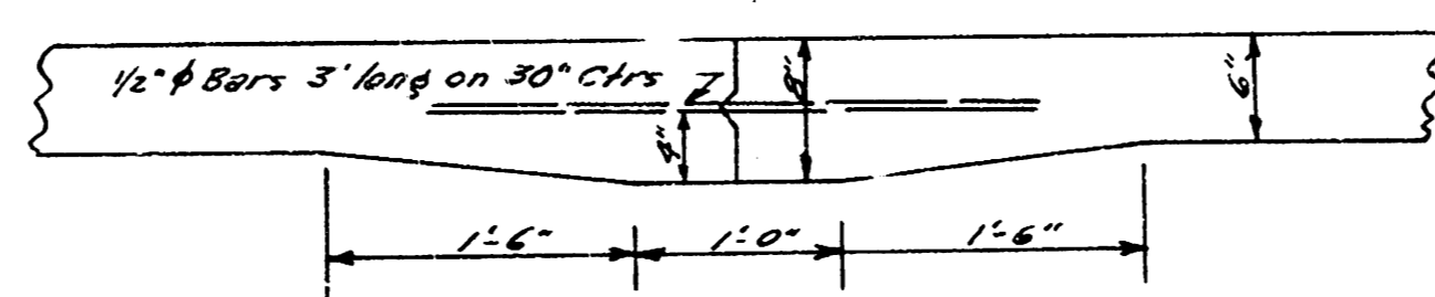
MASTIC JOINT DETAIL NO SCALE
