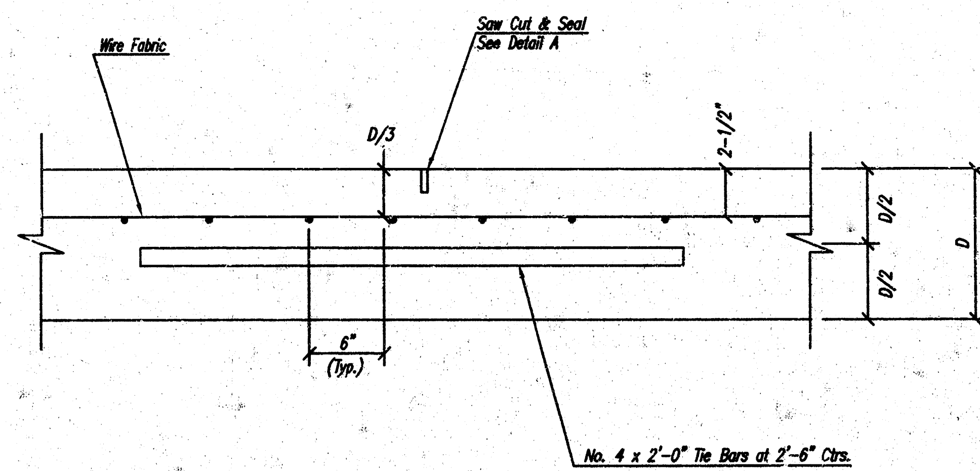
LONGITUDINAL JOINT DETAIL (L.J.)
