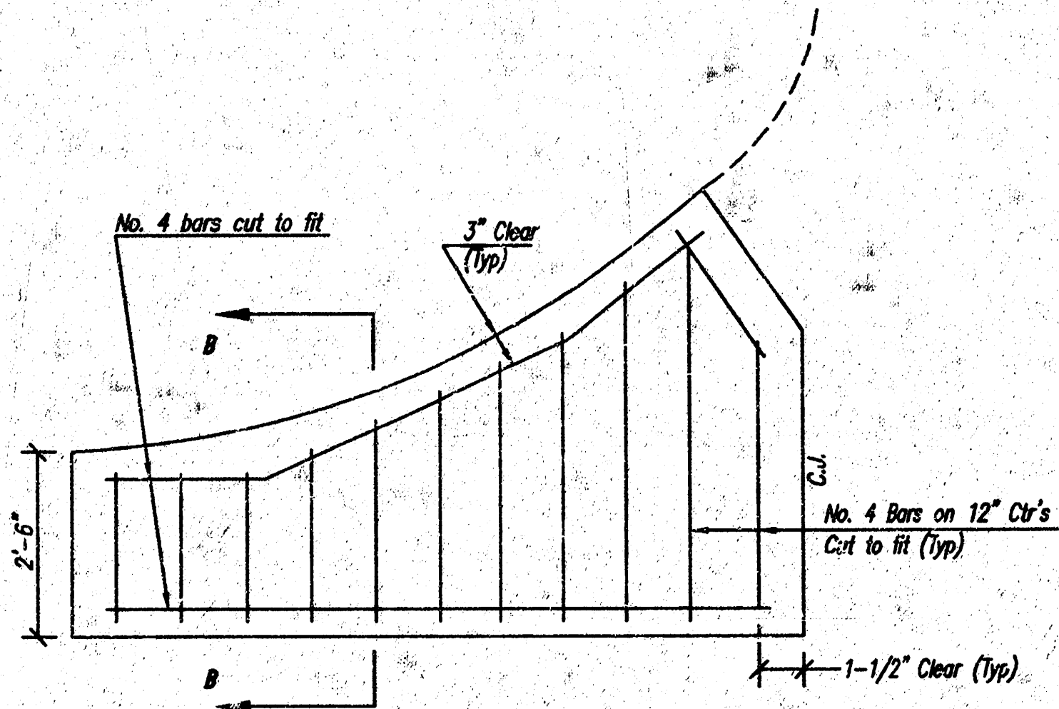
WING REINFORCING DETAIL
