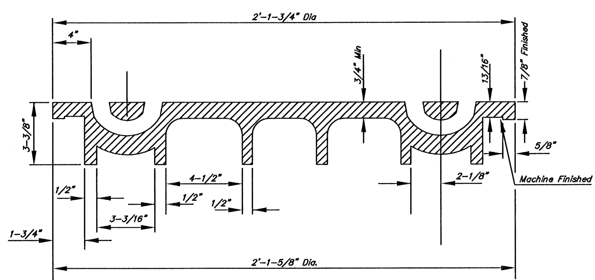
SECTION VIEW
