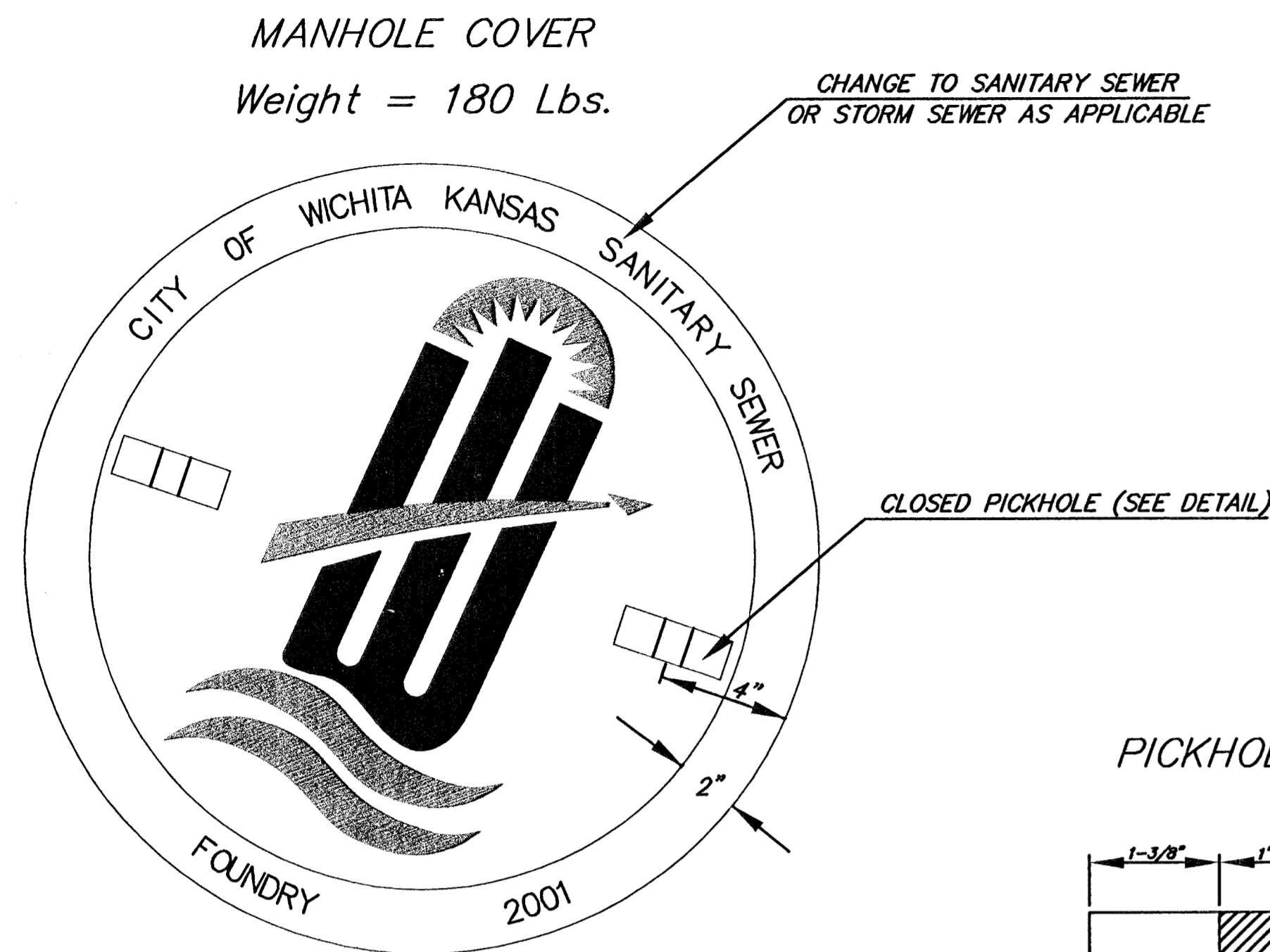
TOP VIEW
