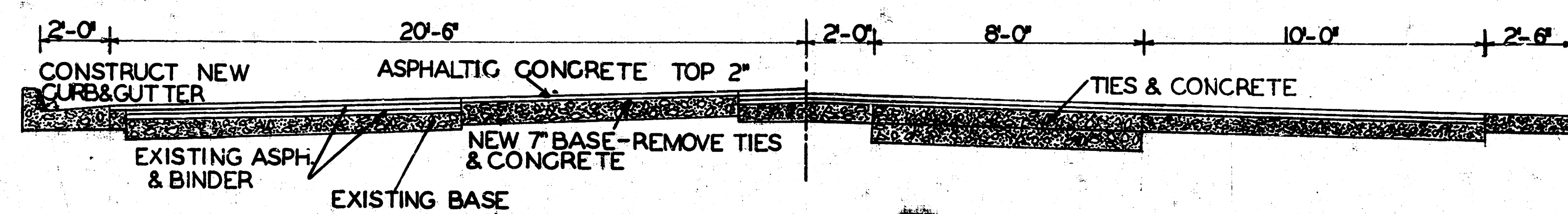
PROPOSED CROSS SECTION
