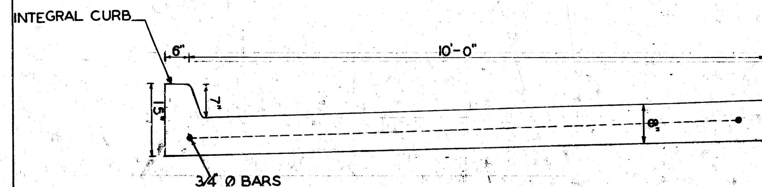
CURB & GUTTER DETAIL FOR BUS STOPS SCALE 1"=1'-0"
