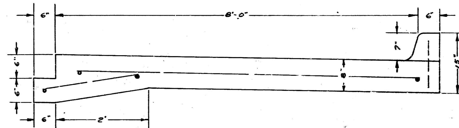
WIDENING DETAIL SCALE 1" = 1'
