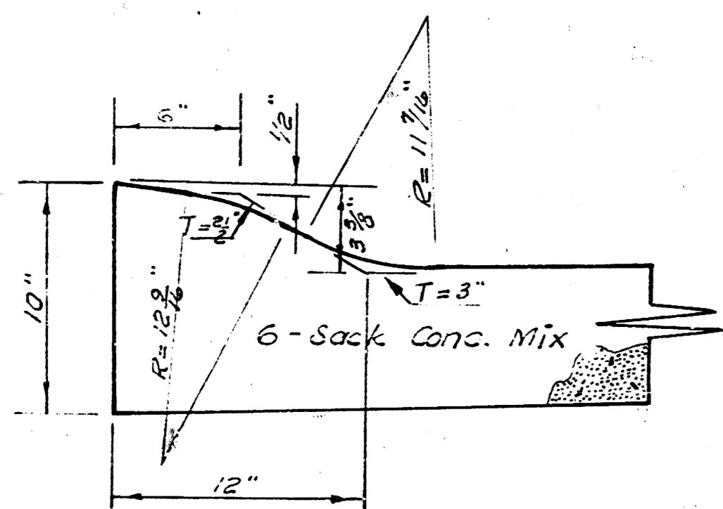
ROLL CURB DETAIL
