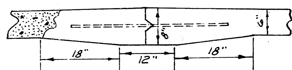
Use #4 Bars, 3' Long on 2'-6" Ctrs. DETAIL OF MASTIC JOINT
