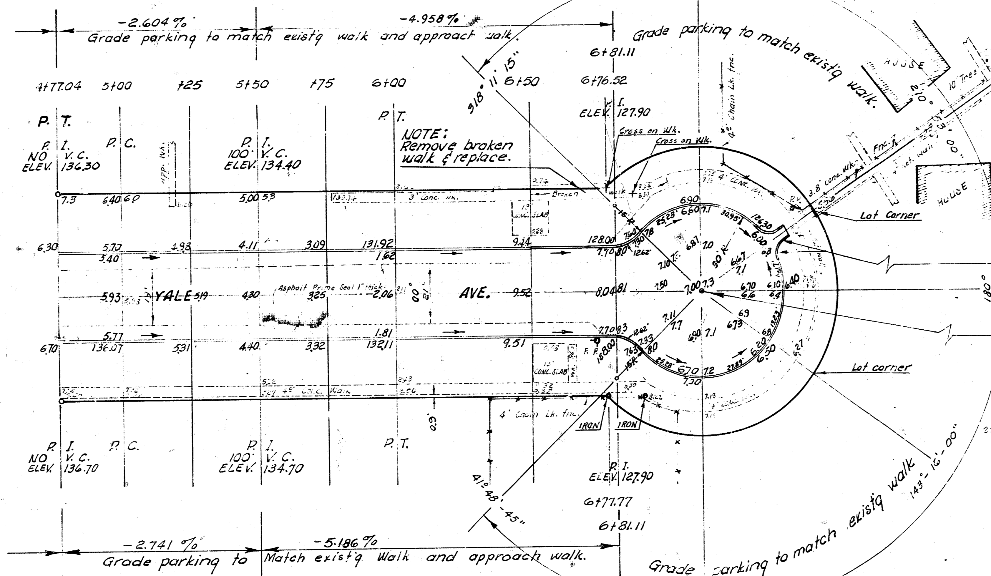
ROLL CURB DETAIL
