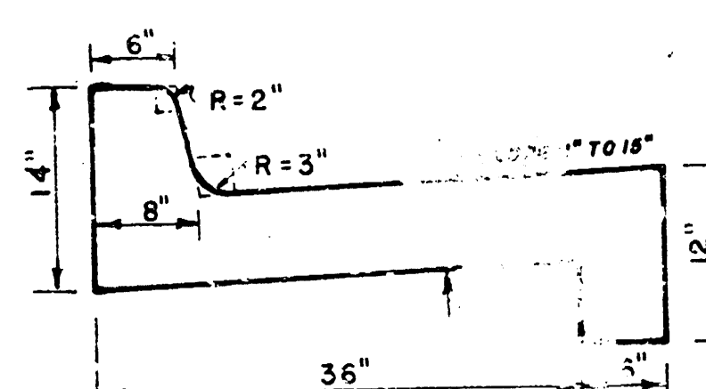
COMBINED CURB & GUTTER SECTION
