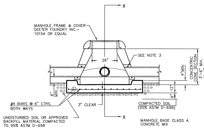
SPECIAL SHALLOW TYPE "P" MANHOLE
