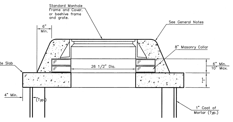
MASONRY COLLAR DETAIL
