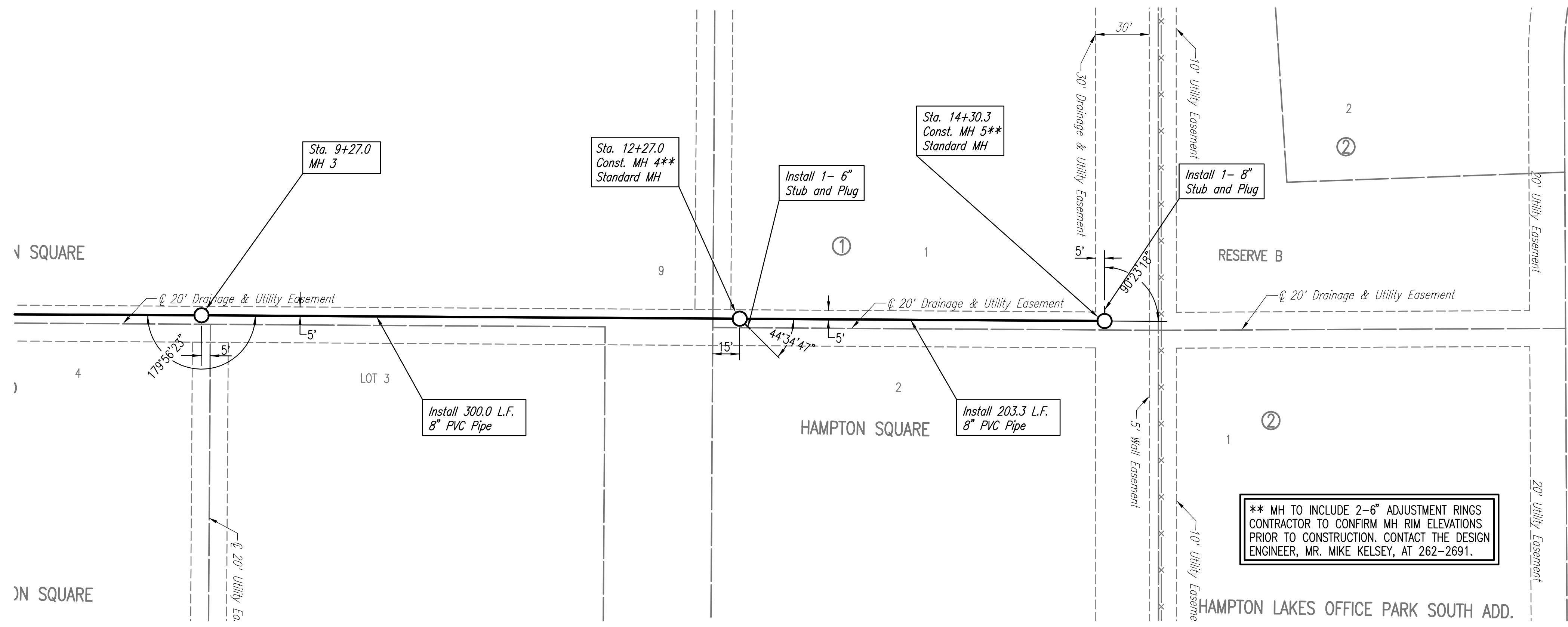
SANITARY SEWER LINE NO. 1
