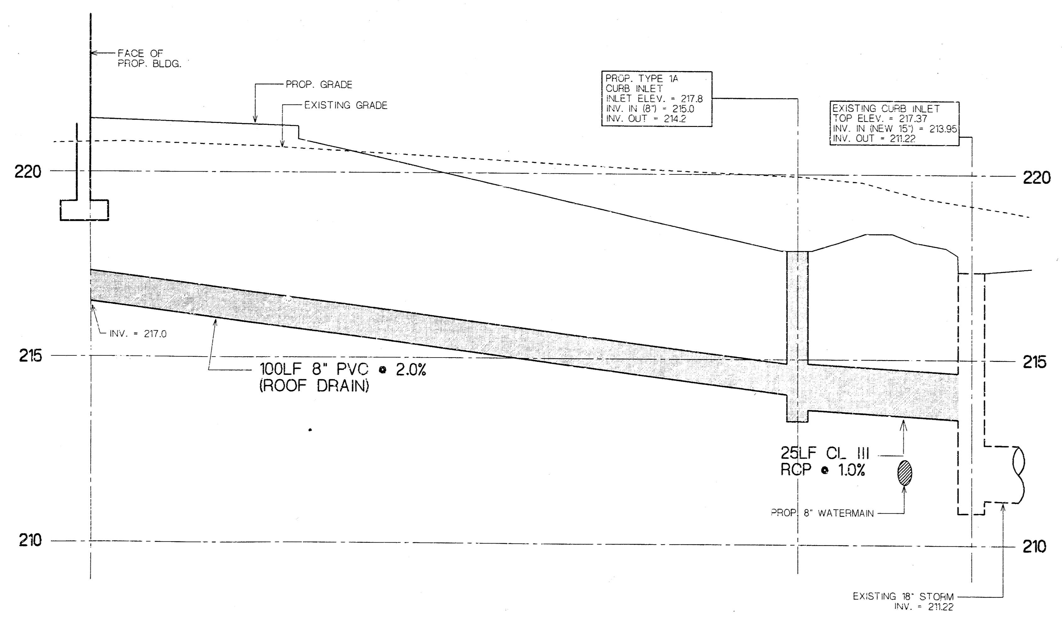
18 STORMSEWER PROFILE #2 12345.678
