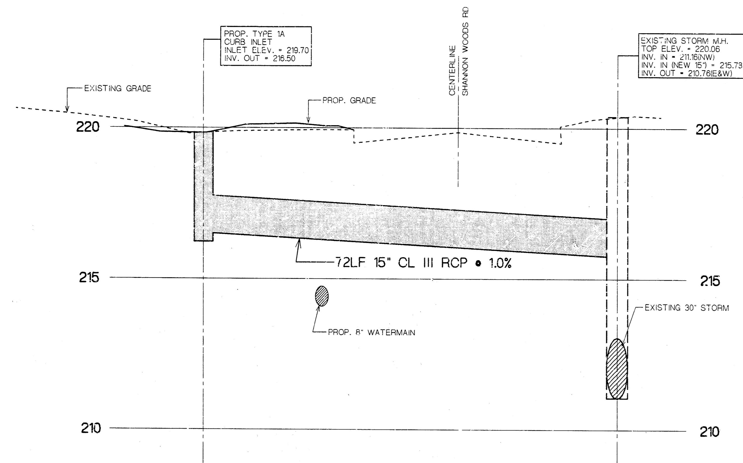
17 STORMSEWER PROFILE #1 12345.678
