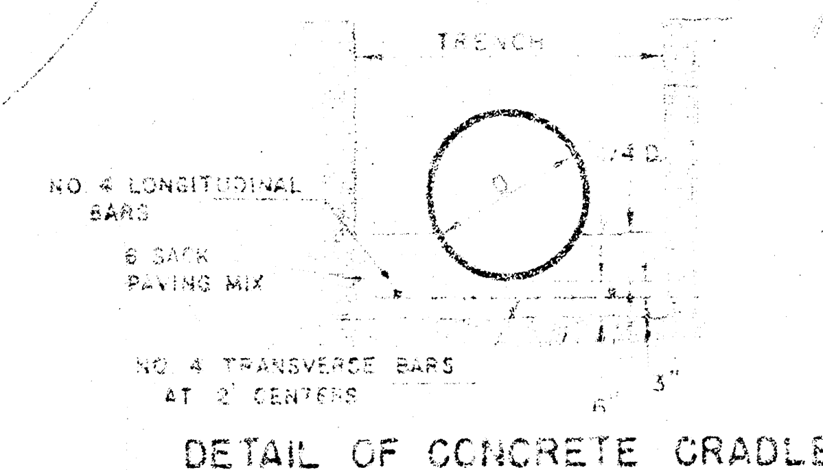
DETAIL OF CONCRETE CRADLE
