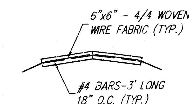
SECTION E-E
