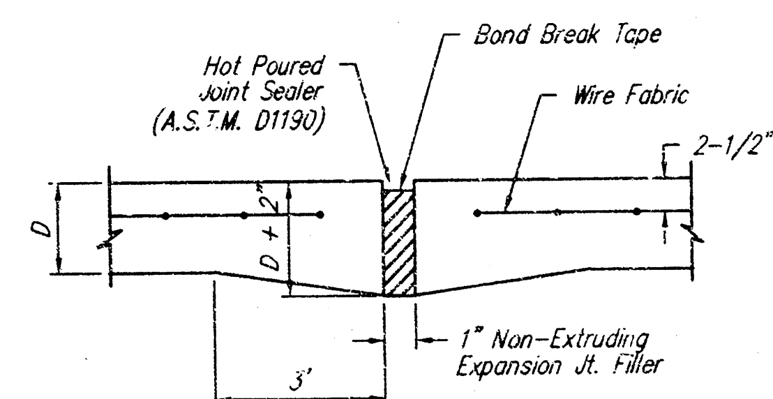
EXPANSION JOINT
