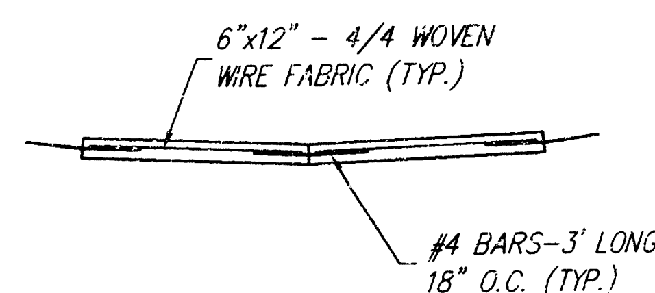
SECTION C-C
