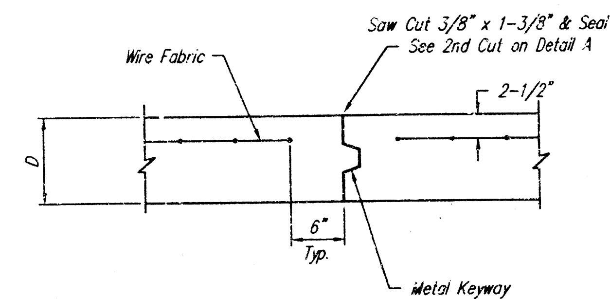
OPTIONAL CONTRACTION JOINT
