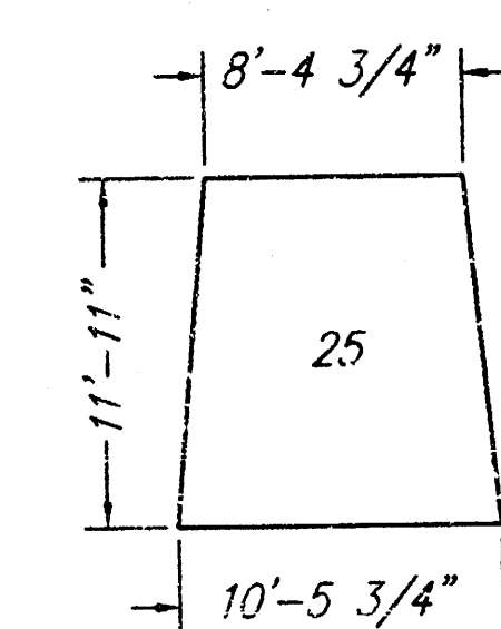
PANEL DESIGN FOR PANELS 25-32
