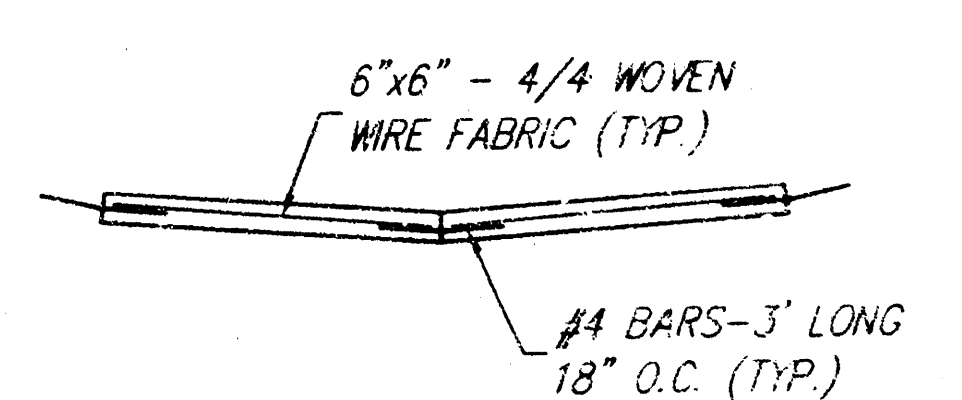
SECTION F-F
