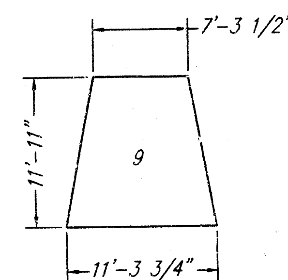
PANEL DESIGN FOR PANELS 9-12
