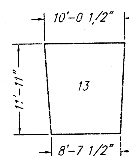
PANEL DESIGN FOR PANELS 13-24
