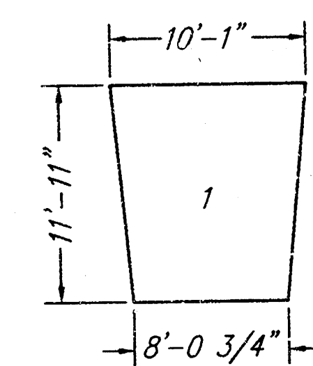
PANEL DESIGN FOR PANELS 1-8
