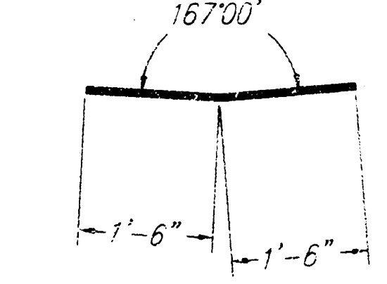
BENDING DIAGRAM
