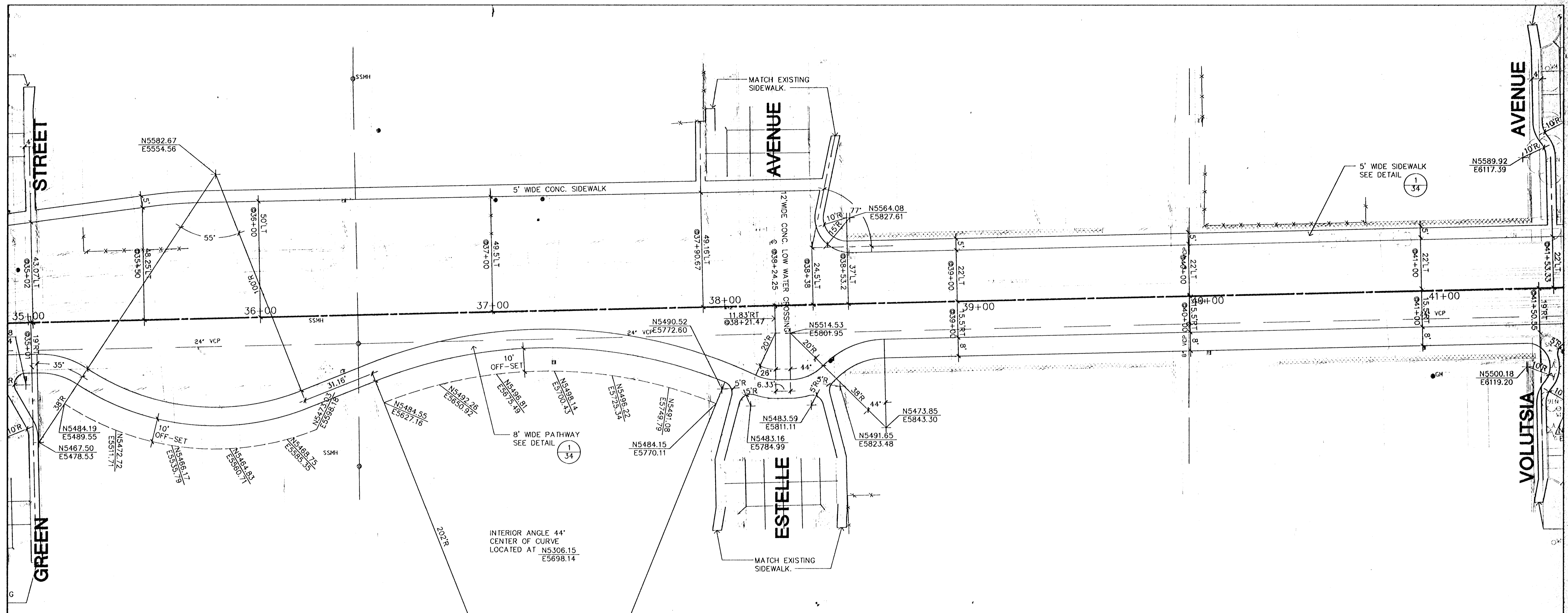
A STATION 35+00.00 TO STATION 41+00.00 0' 10' 20' 1"=20'-0" N
