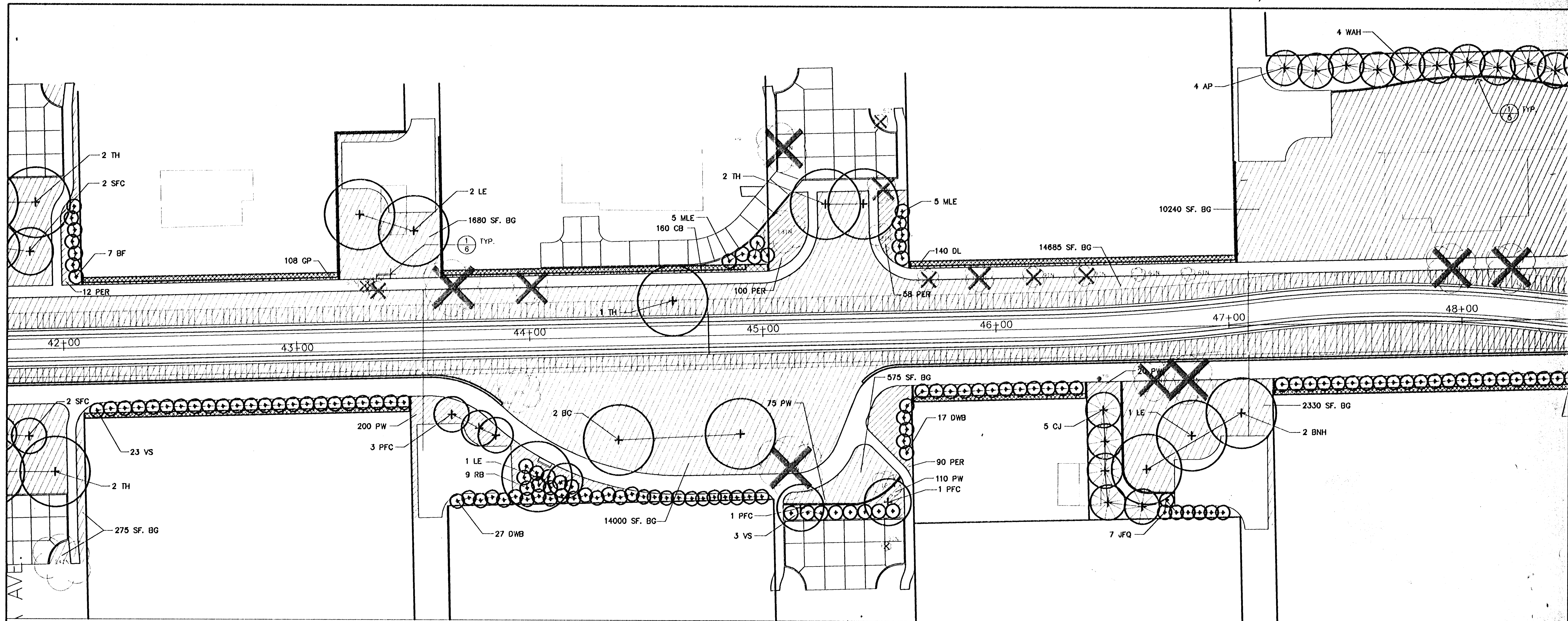
A STATION 41+00.00 TO STATION 48+00.00 0' 10' 20' 1"=20'-0" N
