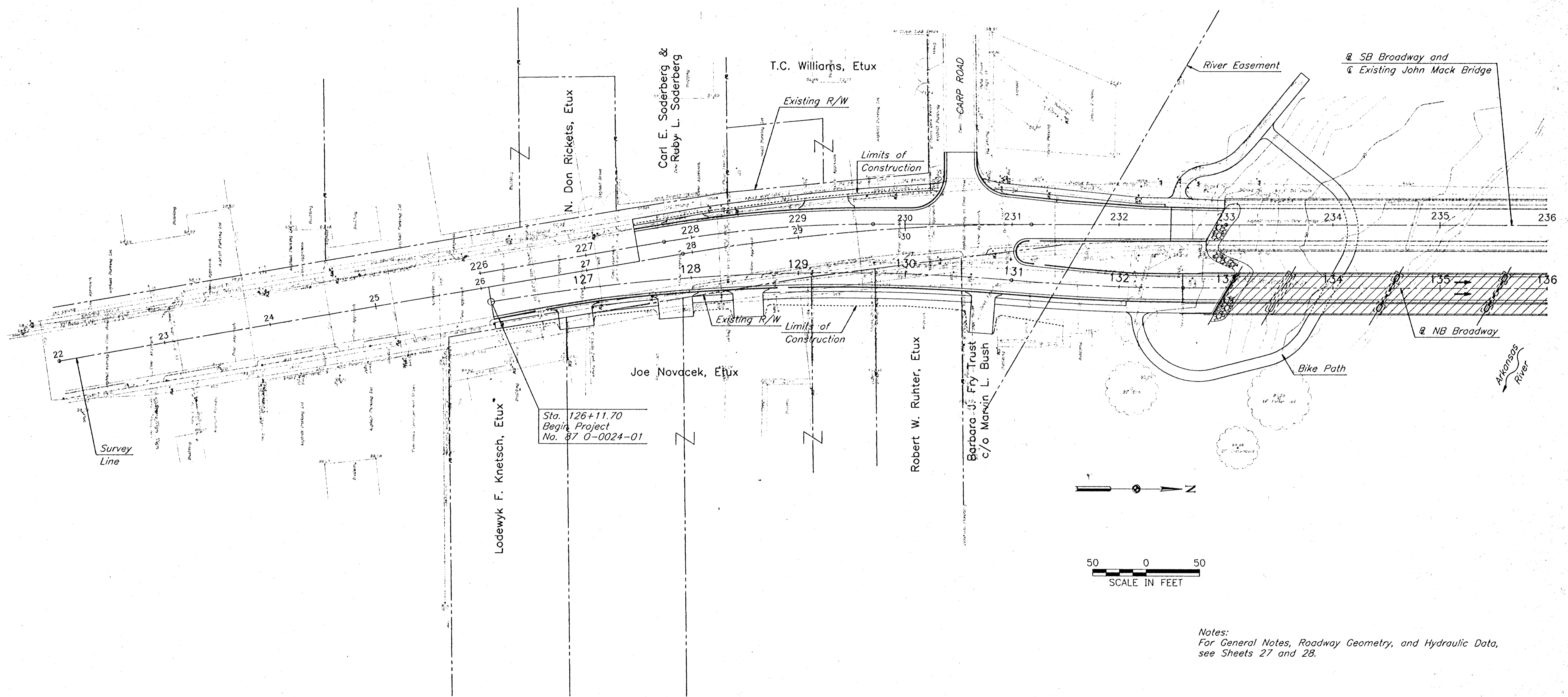
WATERWAY SKETCH AT EXISTING STRUCTURE
