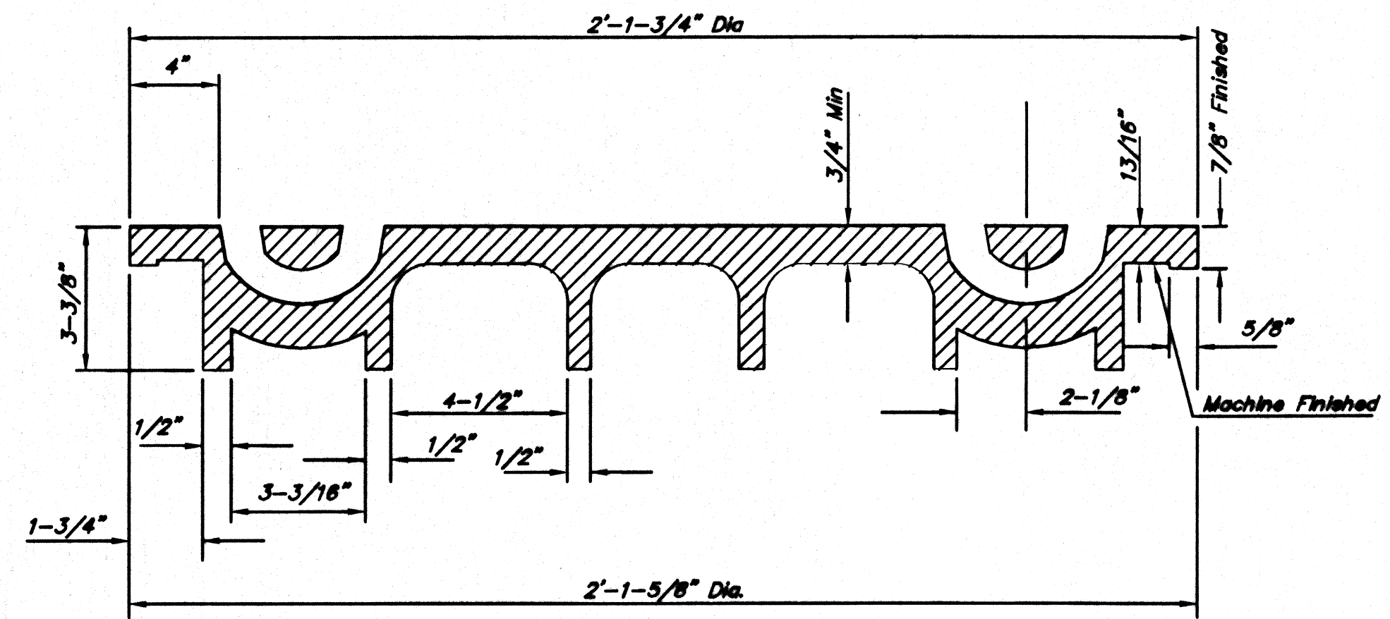
SECTION VIEW
