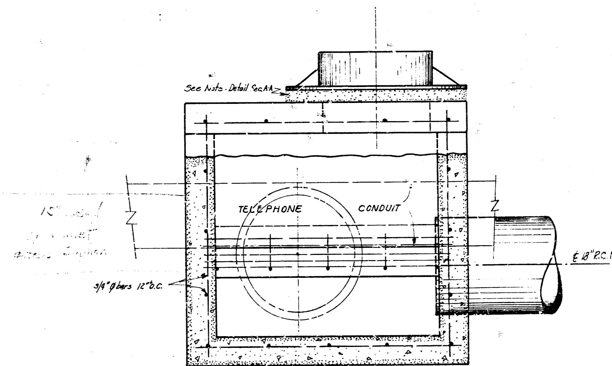
SECTION J-B
