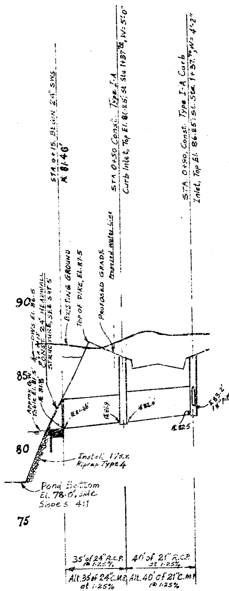
PROFILE OF STORM WATER SEWER LINE 2
