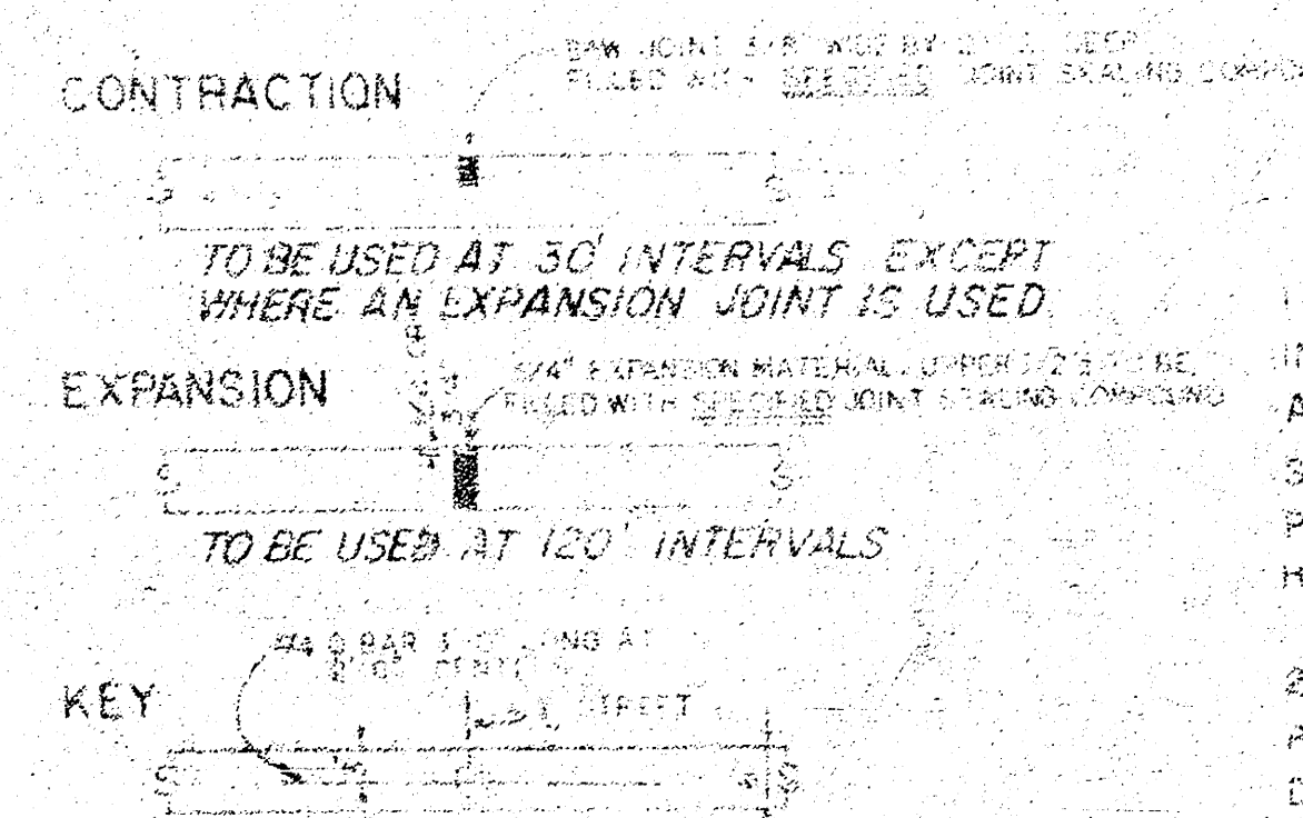
JOINT DETAILS
