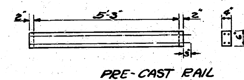
PRE-CAST RAIL
