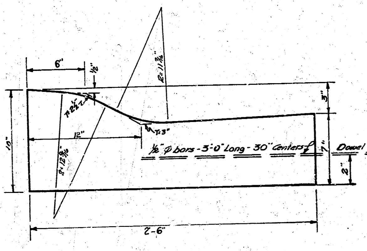
NON-STD. COMB. CURB & GUTTER DETAIL To be poured with sack concrete mix. SCALE: 2"=1'-0"
