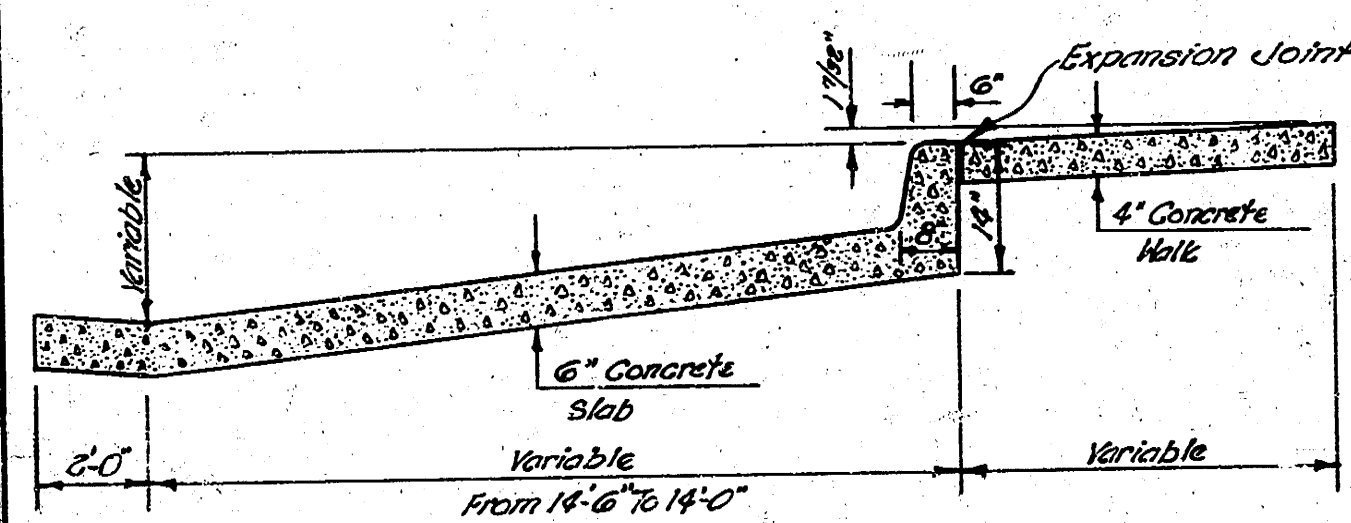
TYPICAL SECTION Not to Scale
